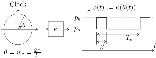
Figure 1: The clock-based switching controller.
