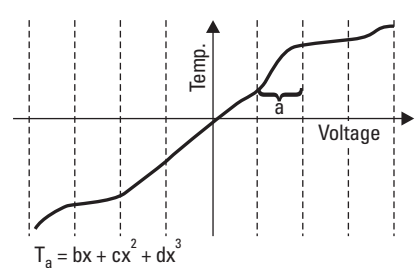
Figure 18 Curve divided into sectors
