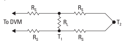
Figure 28 Virtual junction
