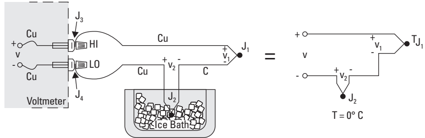
Figure 5 External reference junction
